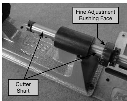
Photo 11. Lubricate Cutter Shaft and Fine Adjustment Bushing Face
