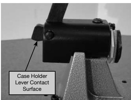
Photo 12. Lubricate Case Holder Lever
